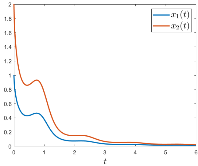
Figure 2: The graphs of the solutions x_1 and x_2 to the example from eq. (5.1).
