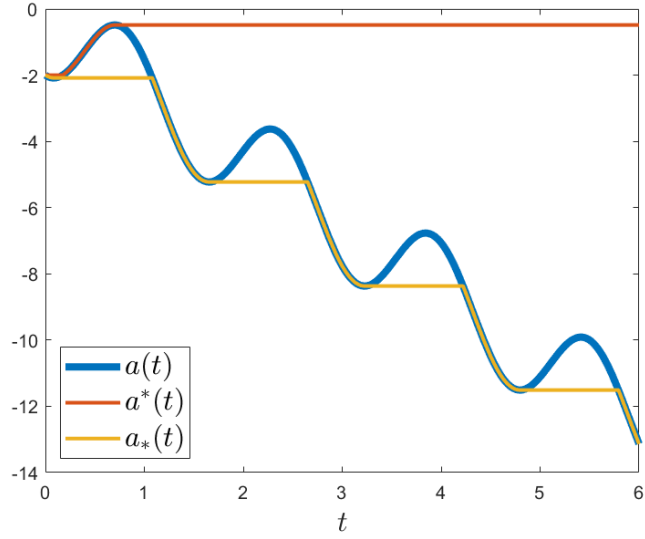
Figure 1: The functions a(t) , a_*(t) and a^*(t) for the example from eq. (5.1).
