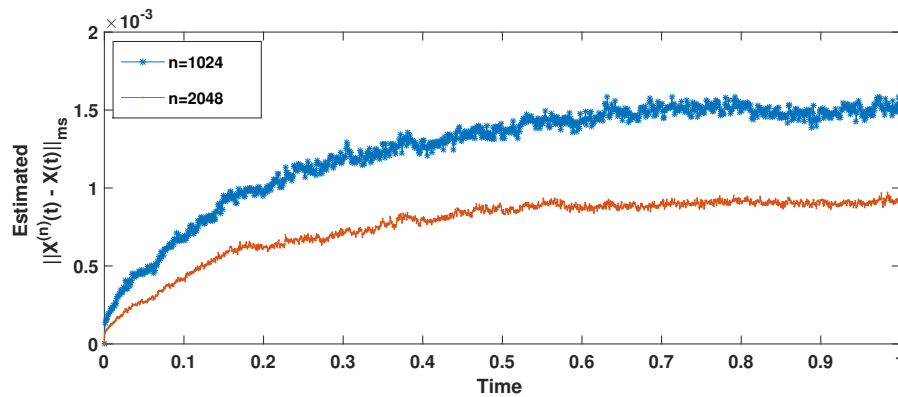
Figure 1: Estimated errors for Equation (32)
